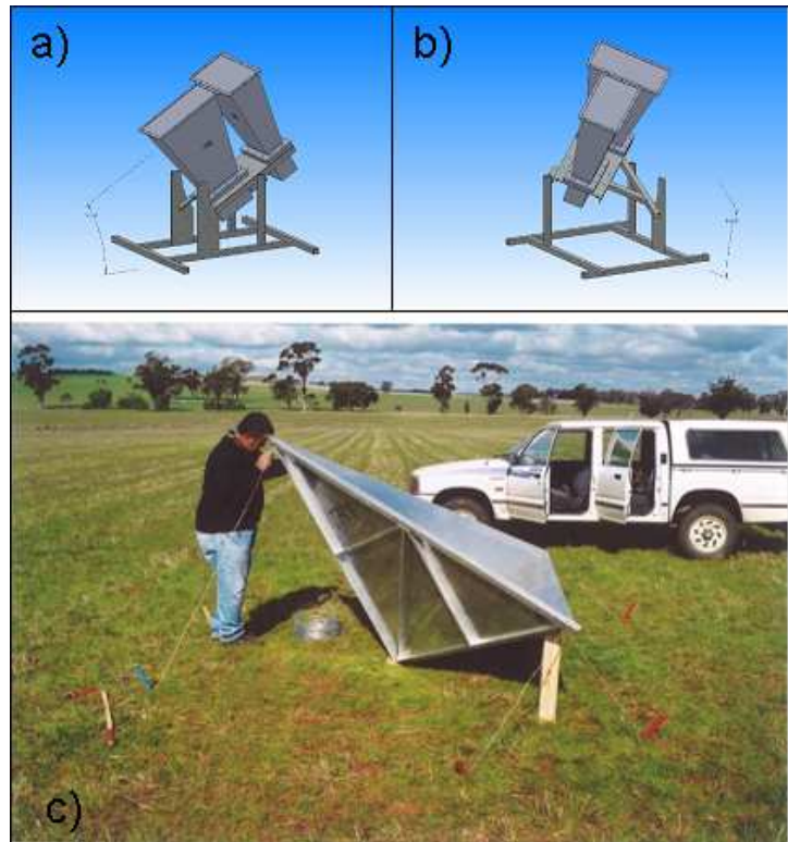
Figure 5-7. Polarimetric Active Radar Calibrators #1 and #2 (a), #3 (b) and Passive Radar Calibrator (c)
