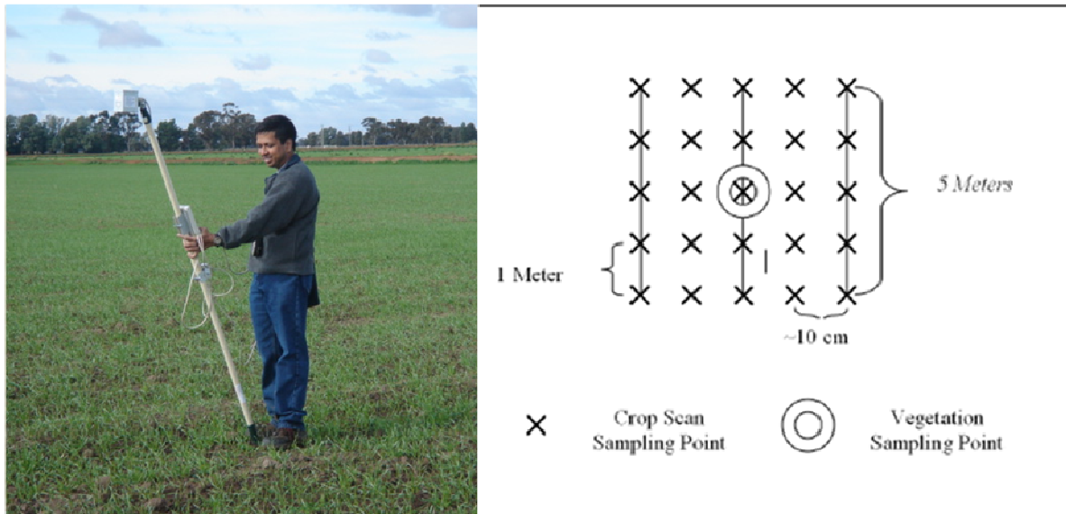
Figure 7-1. (Left) CROPSCAN Multispectral Radiometer (MSR). Size is 8cm × 8cm × 10 cm. (Right) Illustration of the surface reflectance protocol.
