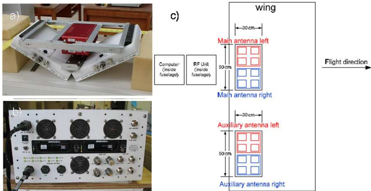
Figure 3-5. View of PLIS antennas (a), RF unit (b) and aircraft configuration (c).
