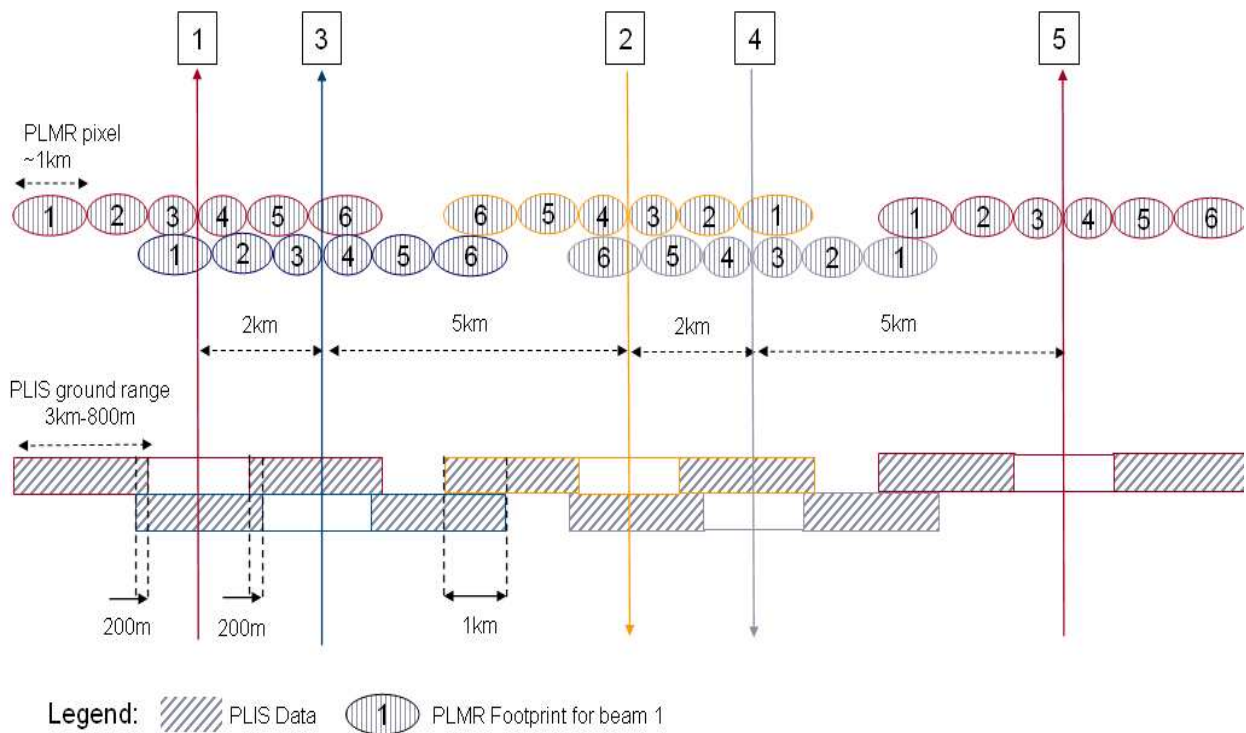
Figure 5-1. Flight line pattern and PLIS/PLMR overlap diagram for SMAPEX regional flights. Different flight lines are indicated by different colours.
