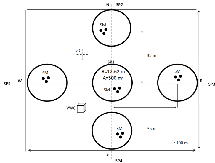
Figure 7-4. Site design for forest sampling (SR-surface roughness, SM-surface moisture, VWC-vegetation water content).
