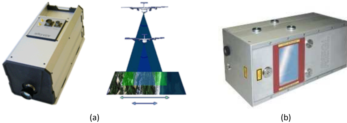
Figure 3-8. (a) AisaHAWK hyperspectral sensor; (b) RIEGL 2D laser scanner
